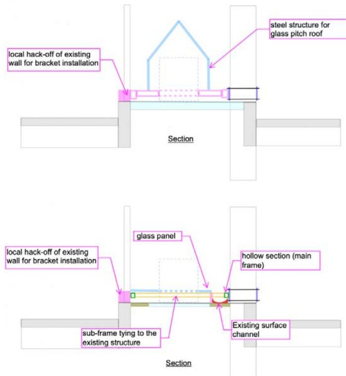
Figure 120 Sectional diagrams for the proposed new fire rated glass panel. (Above: Option E; Below: Option D)
