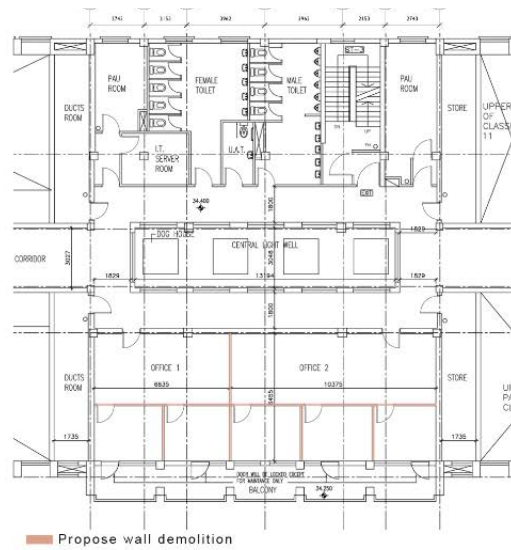
Existing 3/F Part Plan
