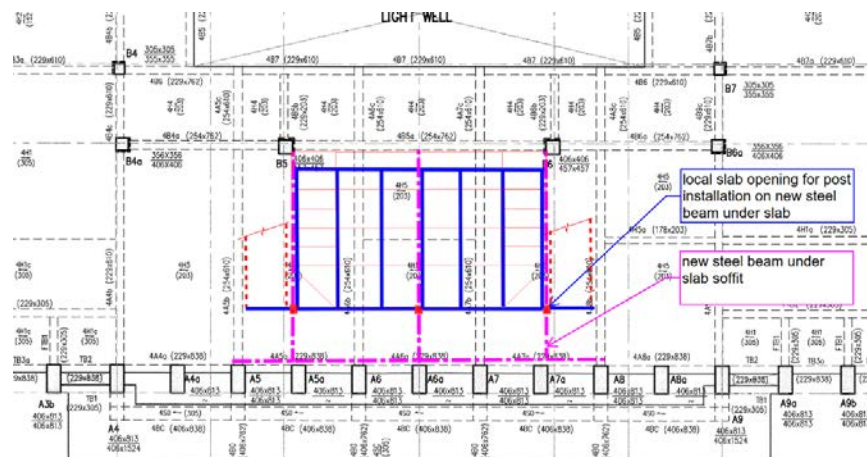
Figure 115 4/F Framing plan (partial) for the proposed removal of slabs. Purple lines: new reinforcement beams for slab opening; blue lines: location of structural beams for new staircase
