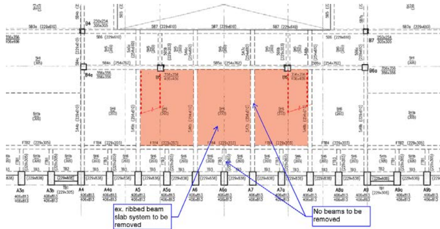
Figure 116 5/F Framing plan (partial) for the proposed removal of slabs.
