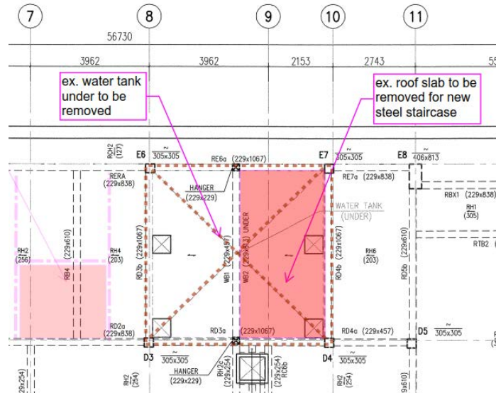
Figure 121 Roof framing plan (partial) for the proposed extension of staircase. Brown dotted lines: location of existing water tank Red shade: location of existing roof slab to be removed
