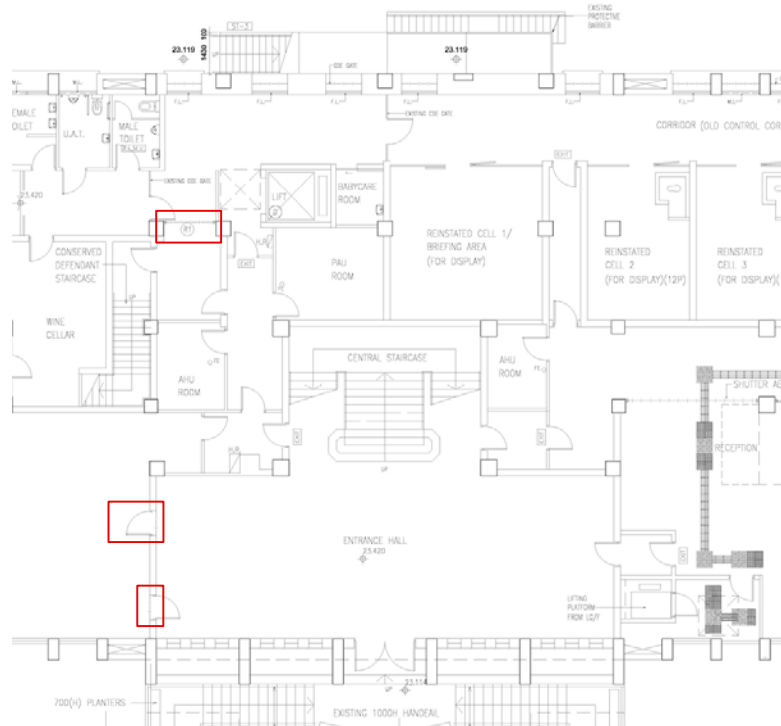
Figure 104 Location of fire shutters on G/F.
