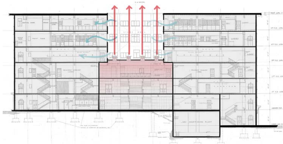
Figure 82 Ventilation diagram of the Central Lightwell.
