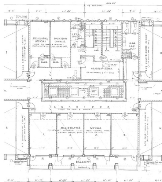
Figure 95 1960s 3/F Part Plan Grid 5-11.
