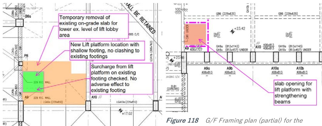
Figure 117 LG/F Framing plan (partial) for the proposed new BFA lifting platform.
