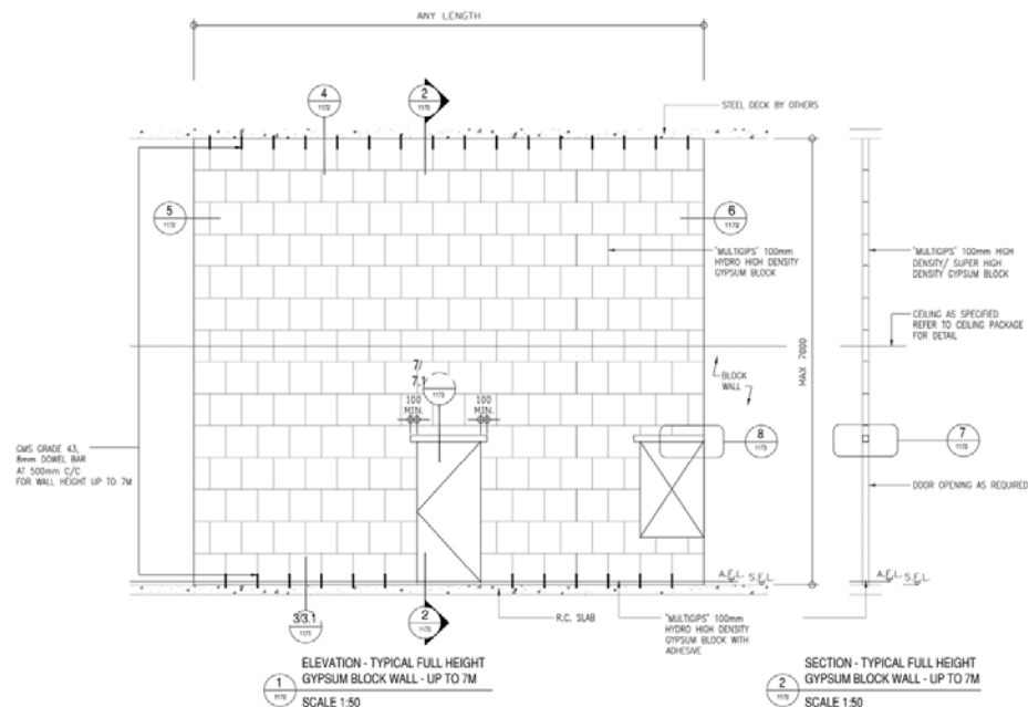
Figure 124 Proposed installation details of the re-partitioning works.
