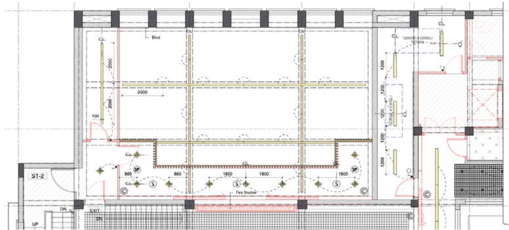
Figure 88 Proposed reflected ceiling plan of Court No.2.
