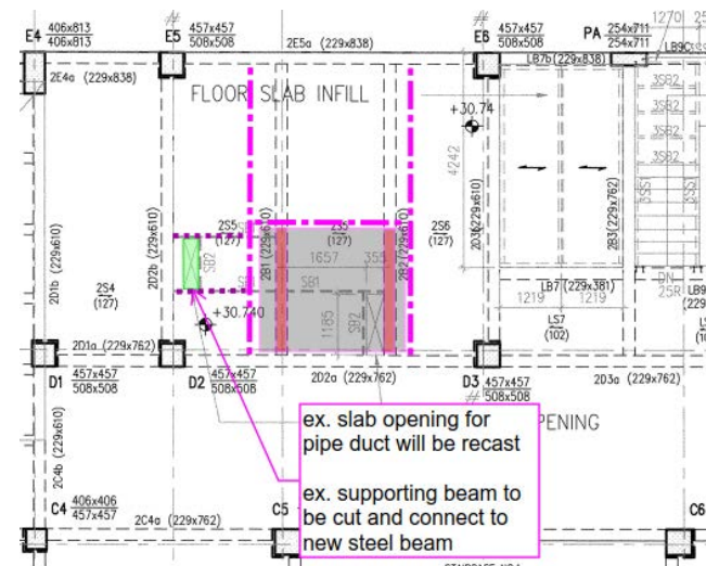
Figure 126 2/F Framing plan (partial) for the proposed works
