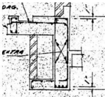
Figure 98 Record drawing of structural detail.
