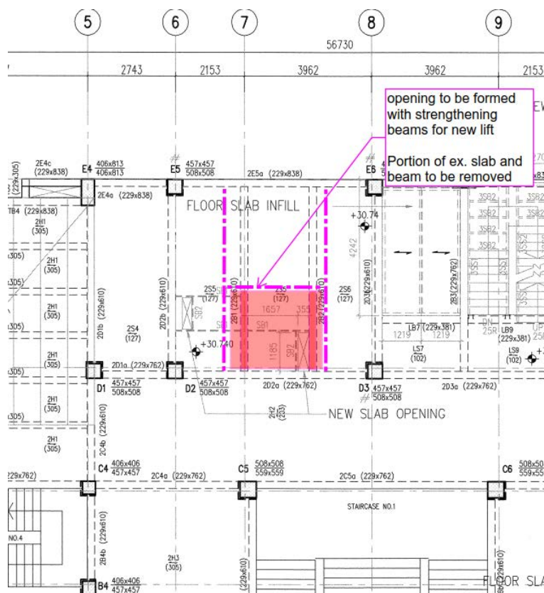
Figure 107 2/F Framing plan (partial) for the proposed new lift.
