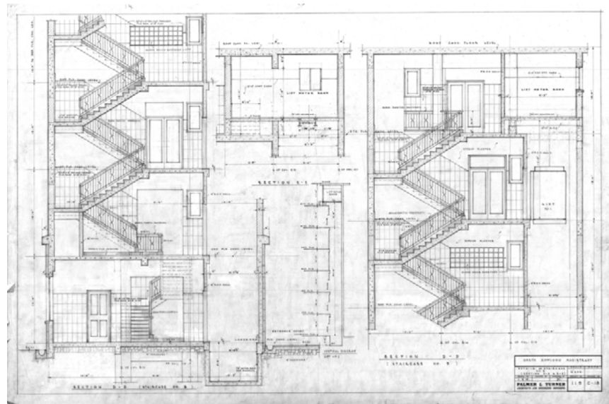
Figure 140 The original design of the Magistrate's Staircase.
