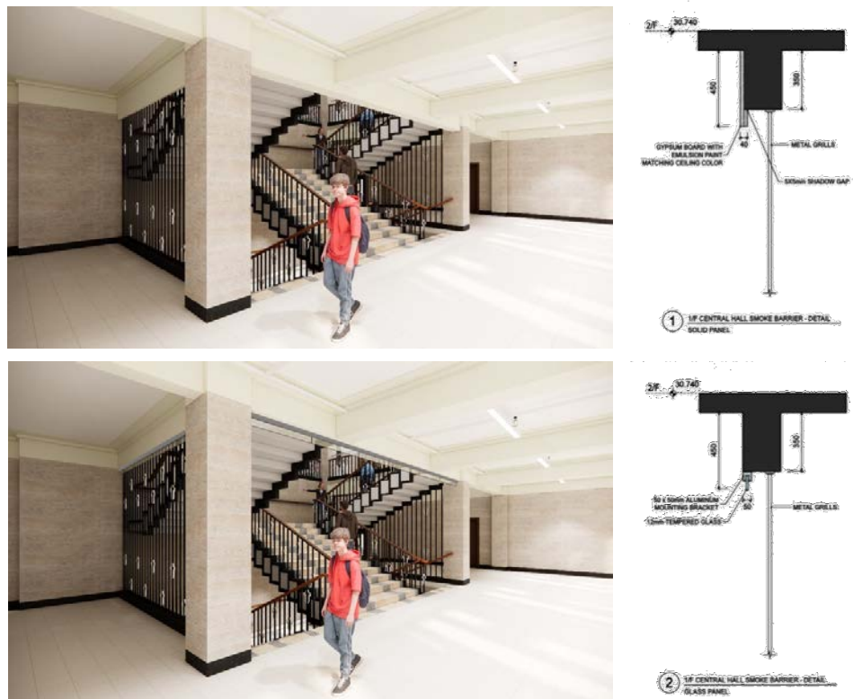
Figure 100 Comparison of smoke barrier design options on 1/F of solid furring (above) and glass panels (below).
