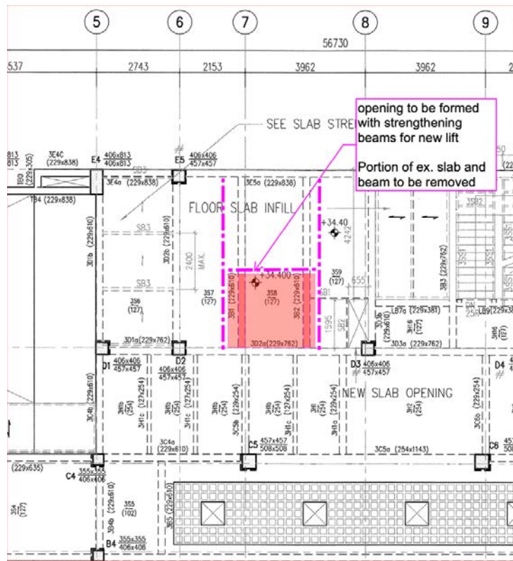
Figure 108 3/F Framing plan (partial) for the proposed new lift. Red shade: Location of lift Red solid: existing beam to be cut and removed Purple line: proposed reinforcement beams
