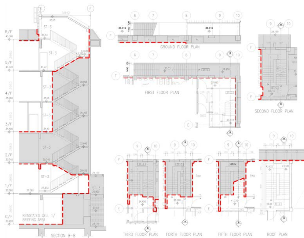
Figure 122 Proposed design of staircase ST-3.
