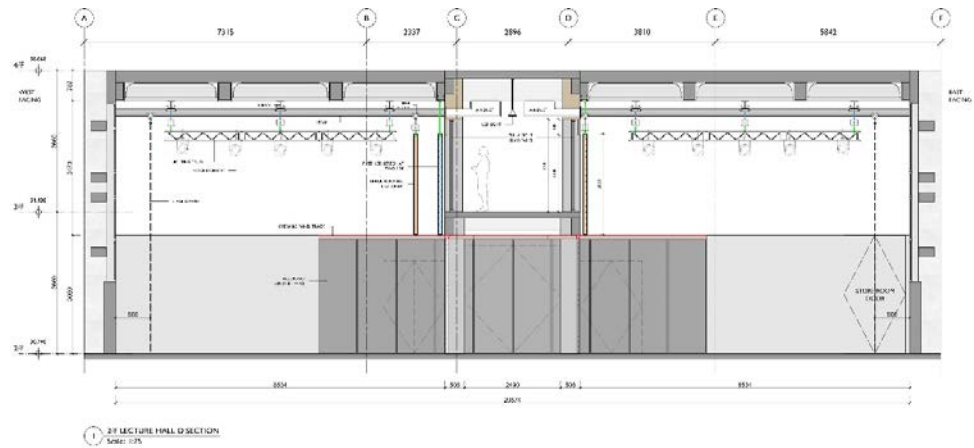
Figure 90 Section of 2/F Lecture Hall D.
