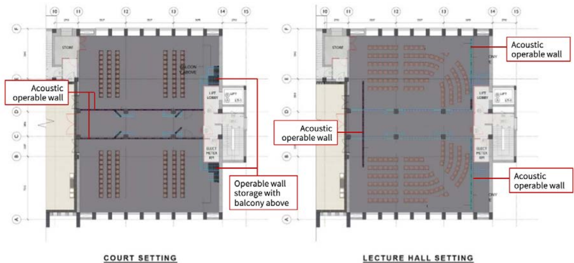
Figure 89 2/F Part Plan Grid 10-15.
