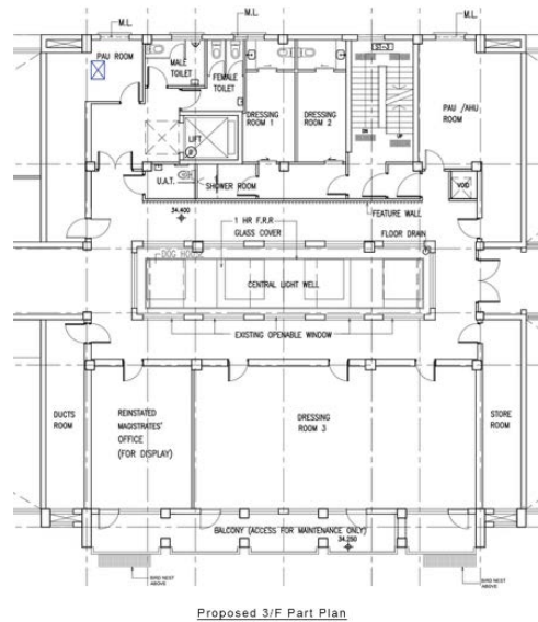
Proposed 3/F Part Plan
