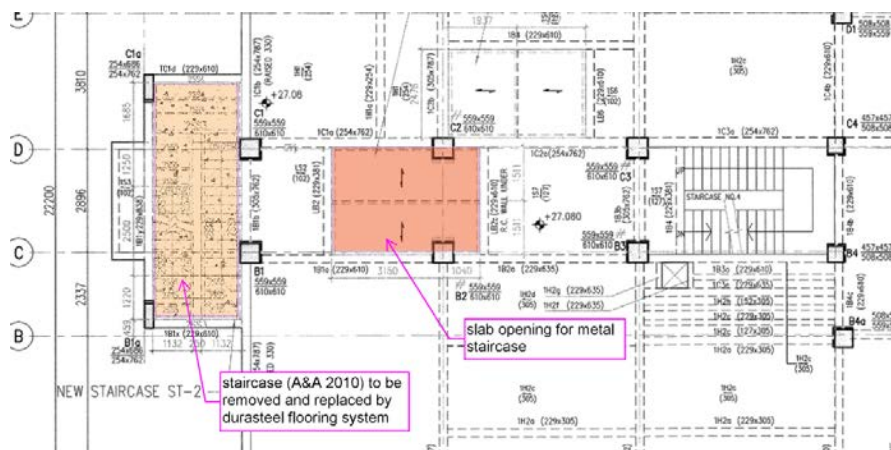
Figure 113 1/F Framing plan (partial) for the proposed alteration of staircases.
