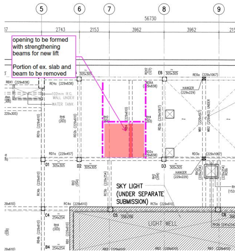
Figure 111 Roof framing plan (partial) for the proposed new lift. Red shade: Location of lift Red solid: existing beam to be cut and removed Purple line: proposed reinforcement beams
