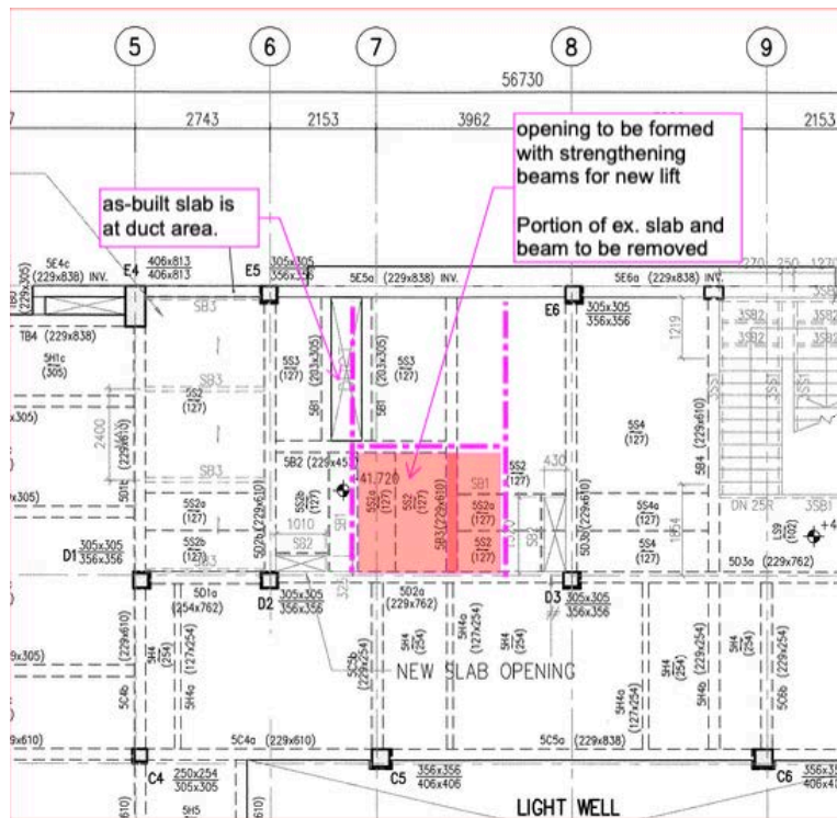
Figure 110 5/F Framing plan (partial) for the proposed new lift. Red shade: Location of lift Red solid: existing beam to be cut and removed Purple line: proposed reinforcement beams
