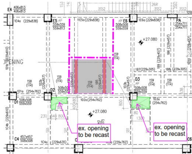
Figure 125 1/F Framing plan (partial) for the proposed works
