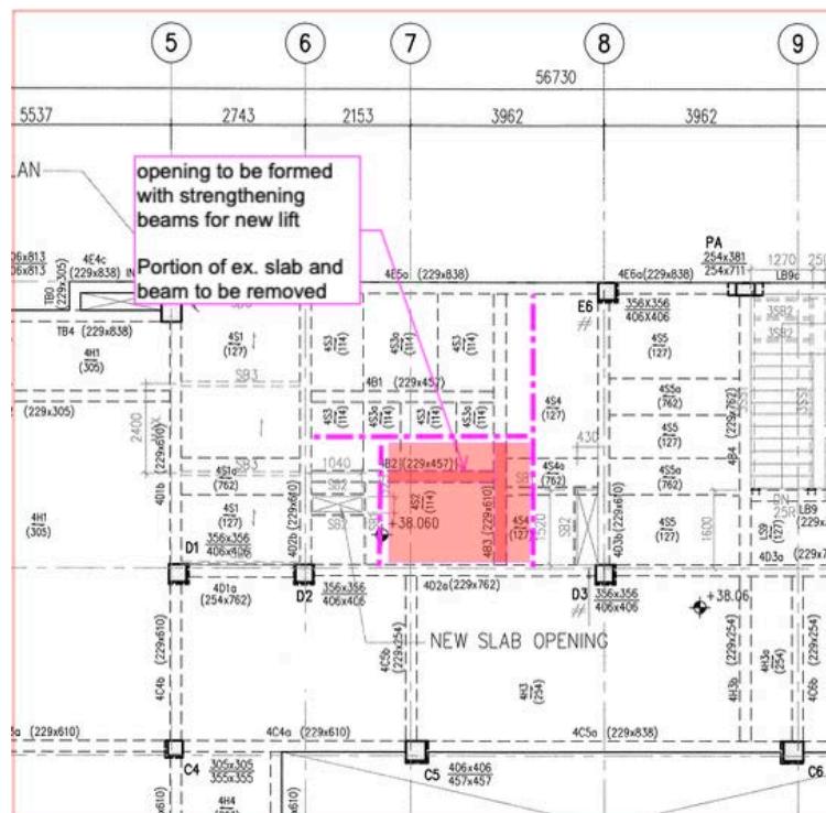
Figure 109 4/F Framing plan (partial) for the proposed new lift. Red shade: Location of lift Red solid: existing beam to be cut and removed Purple line: proposed reinforcement beams
