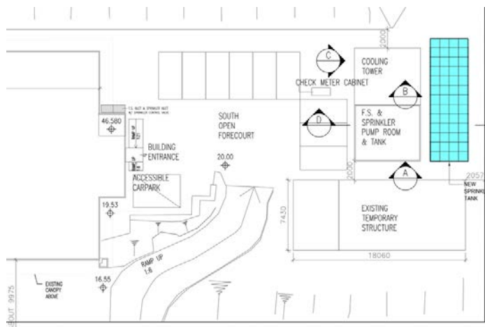
Figure 133 Proposed E&M Layout Plan (South Open Forecourt).
