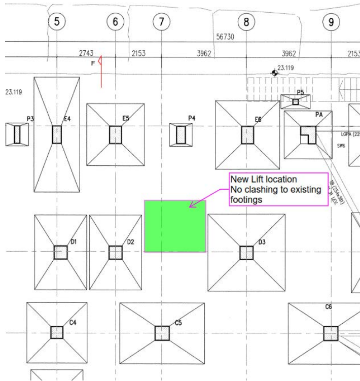
Figure 105 LG/F Framing plan (partial) for the proposed new lift
