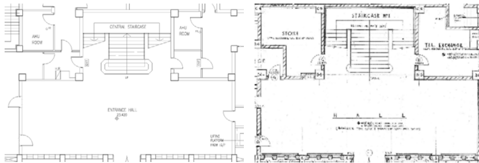
Figure 141 The proposed design (left) and the original design (right) of the Entrance Hall.
