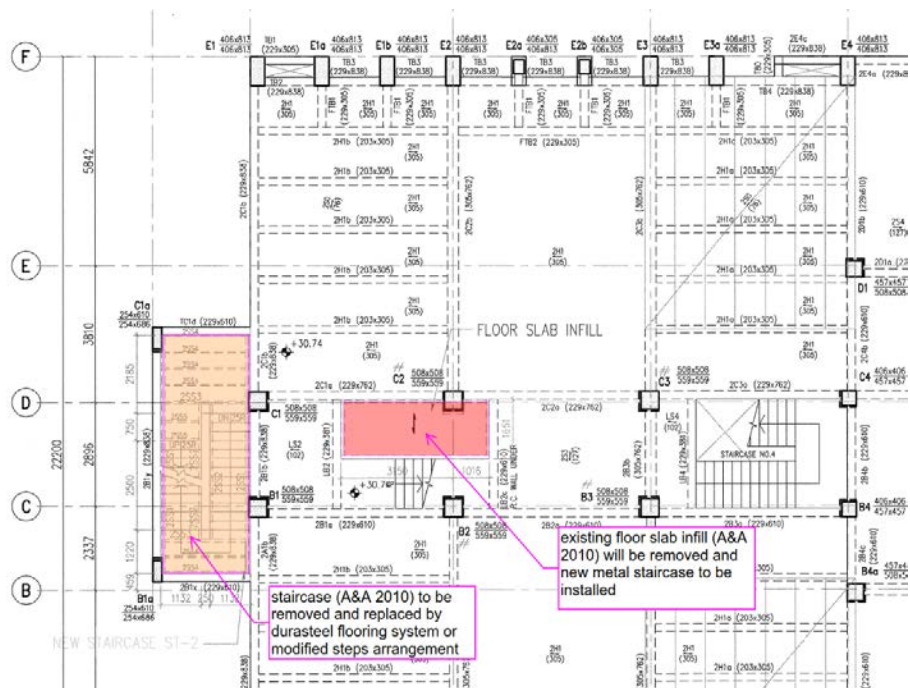
Figure 114 2/F Framing plan (partial) for the proposed alteration of staircases.
