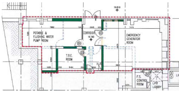
Figure 131 Proposed E&M Layout Plan (LG/F).
