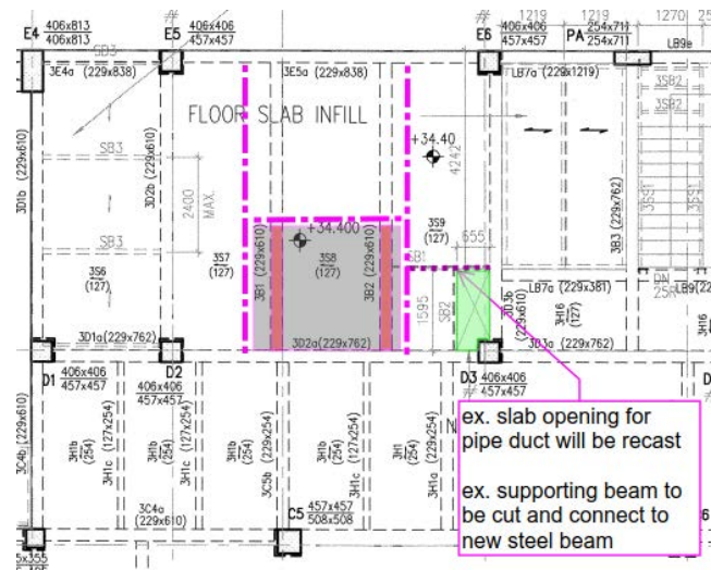
Figure 127 3/F Framing plan (partial) for the proposed works
