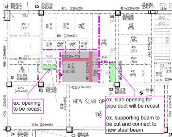
Figure 128 4/F Framing plan (partial) for the proposed works
