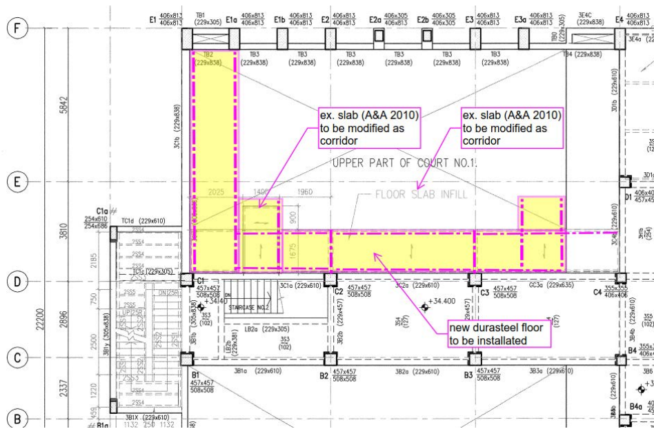
Figure 123 3/F Framing plan (partial) for the proposed new corridor.
